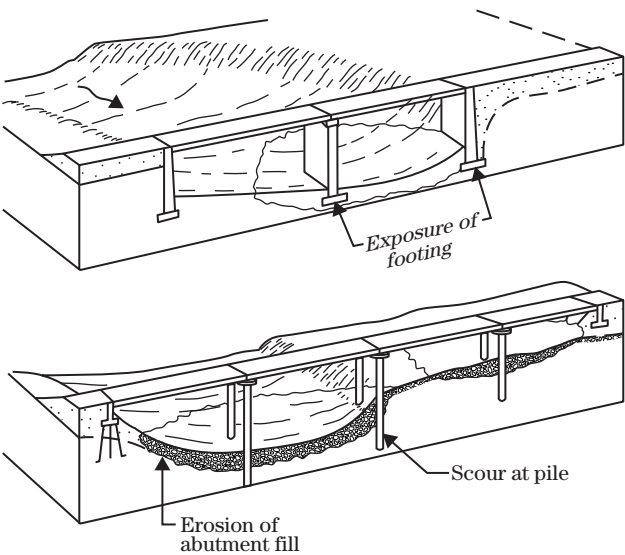
Figure TS14B-3 Examples of general scour
