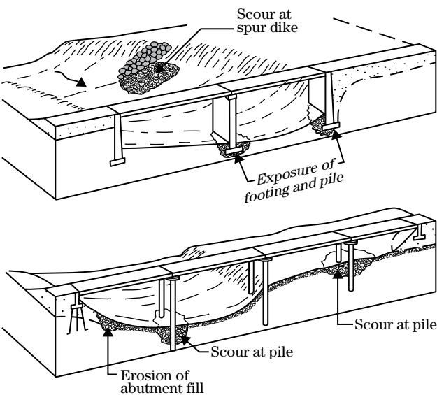
Figure TS14B-2 Examples of local scour
