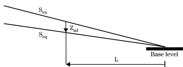
Figure TS14B-6 Definition of equilibrium slope, S_{eq}
